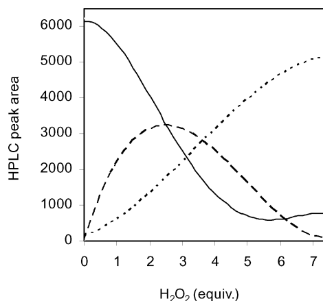
Figure 5. The change in concentration of 5 (—), 21 (---) and 6 (···) with increasing addition of \text{H}_2\text{O}_2 , as 5 is titrated with methyl radicals.
