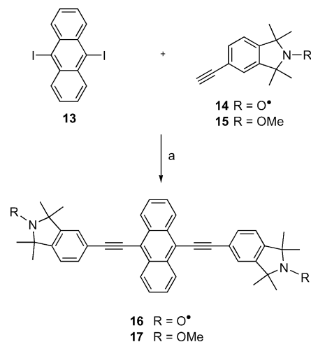
Scheme 4. Reagents and conditions: (a) CuI, PdCl 2 (PPh 3 ) 2 , Et 3 N, 85 °C, 16 h, (for 16 : 67%, for 17 : 98%).
