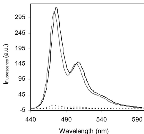
Figure 2. Fluorescence spectra of 9,10-bis(phenylethynyl)anthracene-based probes 16 (···), 17 (—), 19 (···) and 20 (—), 2.5 \mu\text{M} in cyclohexane, following excitation at 430 nm.
