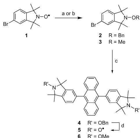
Scheme 1. Reagents and conditions: for 2 : (a) \text{BnCl} , \text{PhNHNH}_2 , t\text{BuOK} , THF, 60%; for 3 : (b) \text{H}_2\text{O}_2 , \text{FeSO}_4 \cdot 7\text{H}_2\text{O} , DMSO, 20 min, 67%; (c) (i) n\text{BuLi} , THF, -78^\circ\text{C} , (ii) anthraquinone, THF, -78^\circ\text{C} to room temp. (iii) \text{SnCl}_2 , \text{AcOH}/\text{H}_2\text{O} , 50^\circ\text{C} , 16 h, for 4 : 36%, for 6 : 38%; (d) (i) \text{Pd/C} , \text{AcOH} , \text{H}_2 (50 psi), 5 h, (ii) \text{PbO}_2 , 30 min, 52%.
