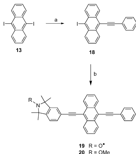
Scheme 5. Reagents and conditions: (a) phenylacetylene, Pd(PPh 3 ) 4 , CuI, Et 3 N, 85 °C, 16 h, 27%; (b) 5-ethynyl-1,1,3,3-tetramethylisindolin-2-yl oxyl 14 or 5-ethynyl-2-methoxy-1,1,3,3-tetramethylisindoline 15 , CuI, PdCl 2 (PPh 3 ) 2 , Et 3 N, 85 °C, 16 h (for 19 : 63%, for 20 : 78%).
